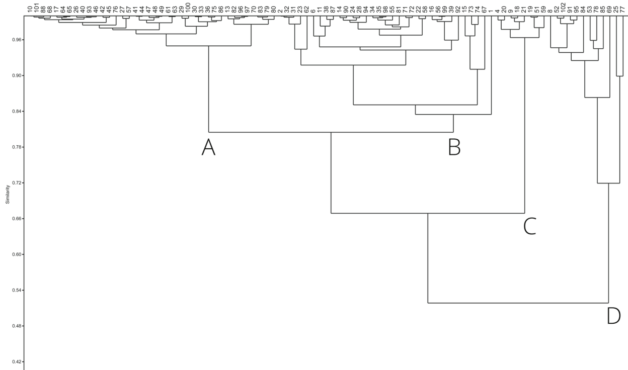
Fig. 8. Results of the cluster analysis for the landform composition of the one-hour catchments of the sites in the study area; four major clusters were set on the similarity level of 80 % (A–C) and 72 % (D Morisita Similarity Index, PAST statistics 3.0); the site numbers are solved in supplementary table (SI 14).
