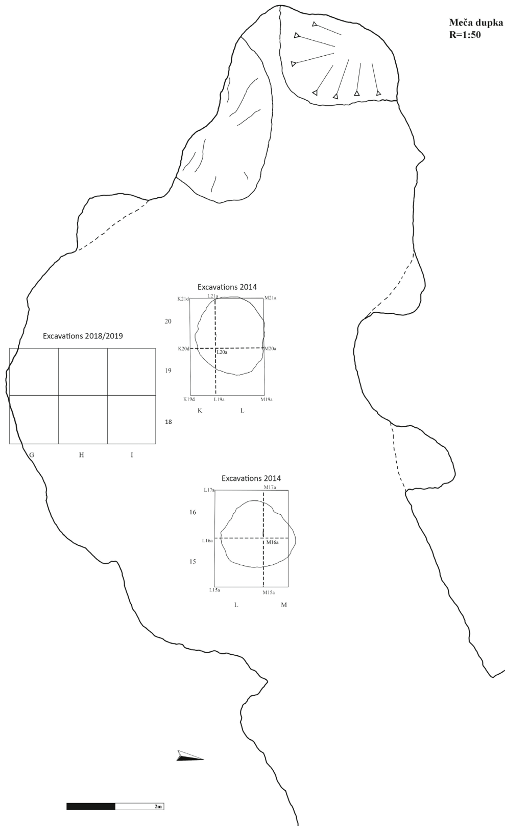
Fig. 2. Map of Meča Dupka showing 2014 and 2018/2019 trenches.
