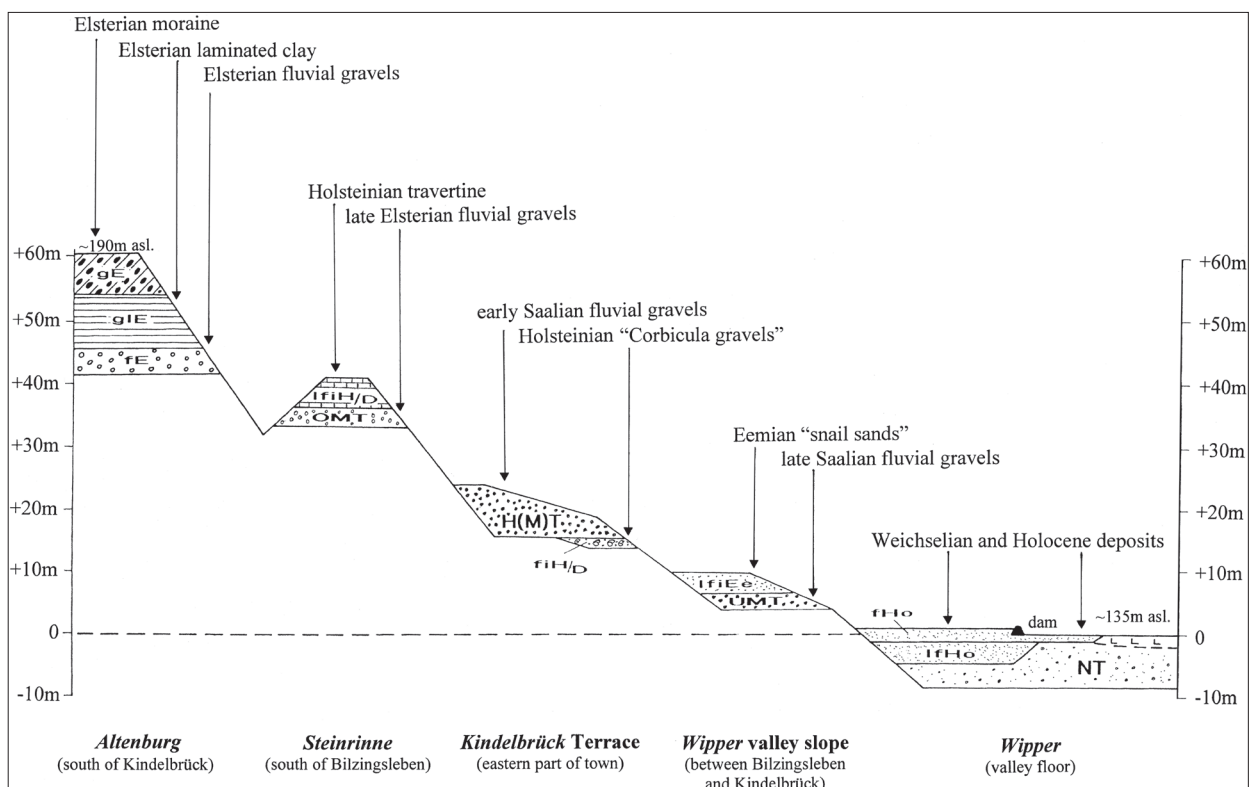
Fig. 8. Synthetic section through the quaternary layers of the lower Wipper valley (adapted from Unger & Kahlke 1995: Abb. 7).
