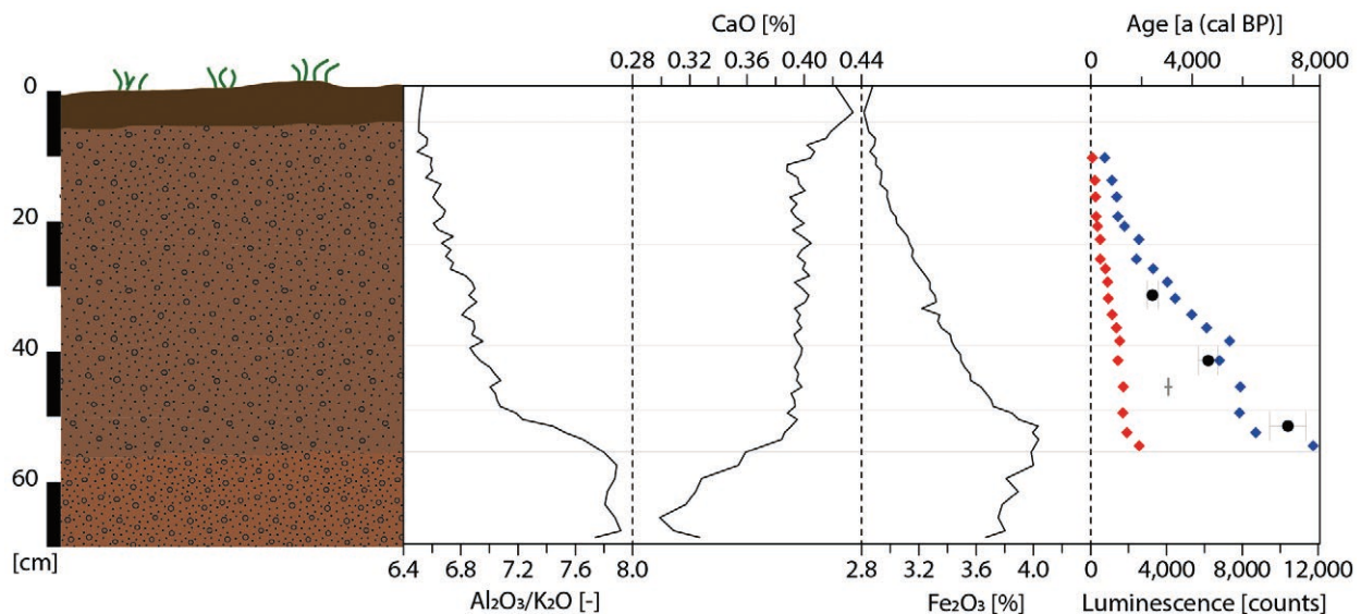
Fig. 3. Geochemical and dating results from Temerești. Solid black lines: geochemical ratios ( \text{Al}_2\text{O}_3/\text{K}_2\text{O} ) and element contents ( \text{CaO} , \text{Fe}_2\text{O}_3 ) as oxides. Red diamonds: luminescence intensities measured by pOSL for IRSL. Blue diamonds: luminescence intensities measured by pOSL for BSL. Gray cross: age range for radiocarbon dating of the charcoal sample found in 46 cm depth. Black circles: OSL ages (error bars indicate 1\sigma uncertainty).
