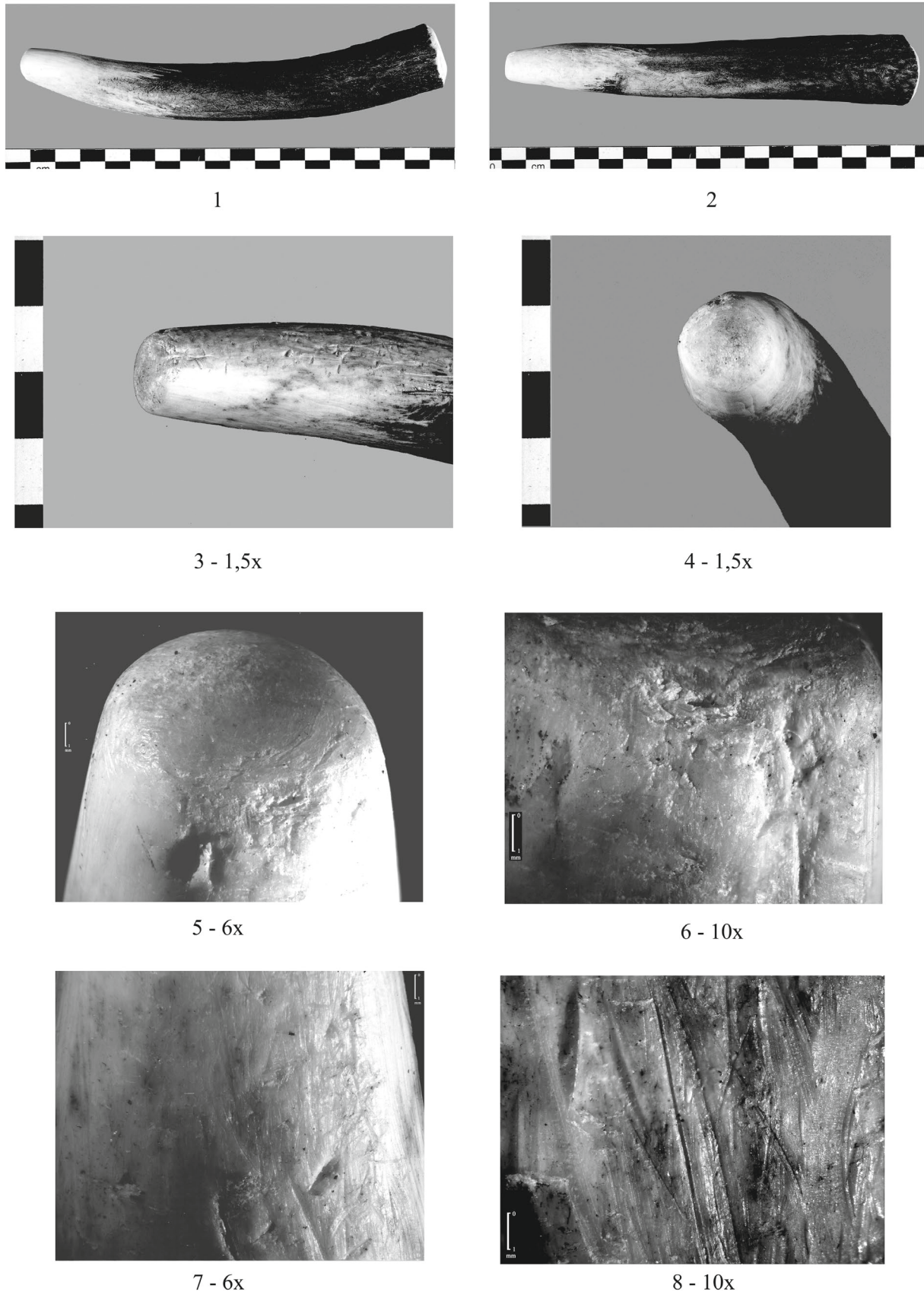
Fig. 6. Experimental antler punch 2, use-wear traces. 1 - right lateral side; 2 - convex side; 3-5 working end and adjacent area of the convex side; 6 - the edge of the working end; 7 - convex side, 1 cm from the tip; 8 - convex side, 5 cm from the tip.
