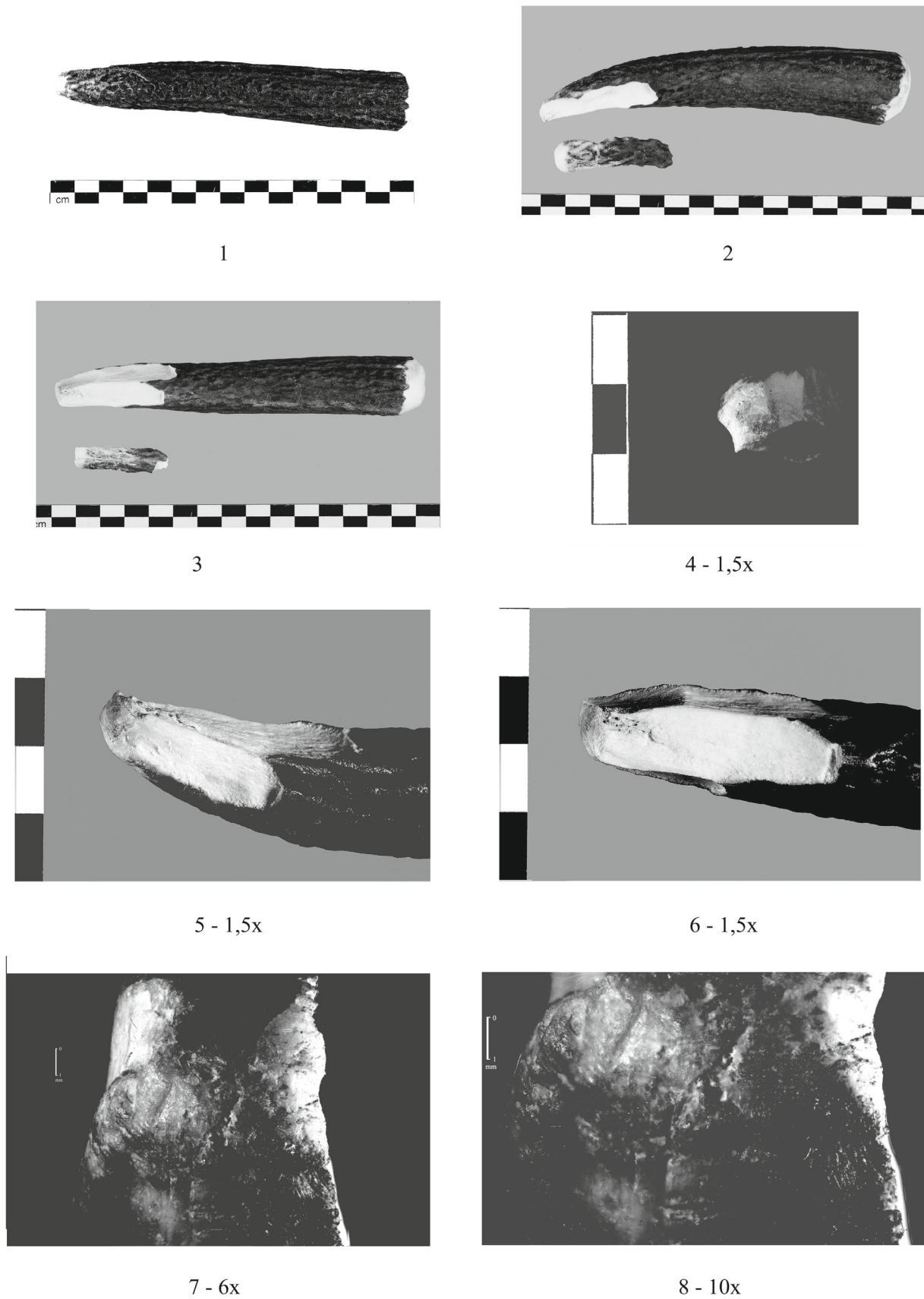
Fig. 4. Experimental antler punch 1, use-wear traces. 1 - convex side; 2 - left lateral side after a long flake vent off; 3 - concave side after another long flake vent off; 4-6 - working end and adjacent area of the convex side; 7-8 - the edge of the working end.
