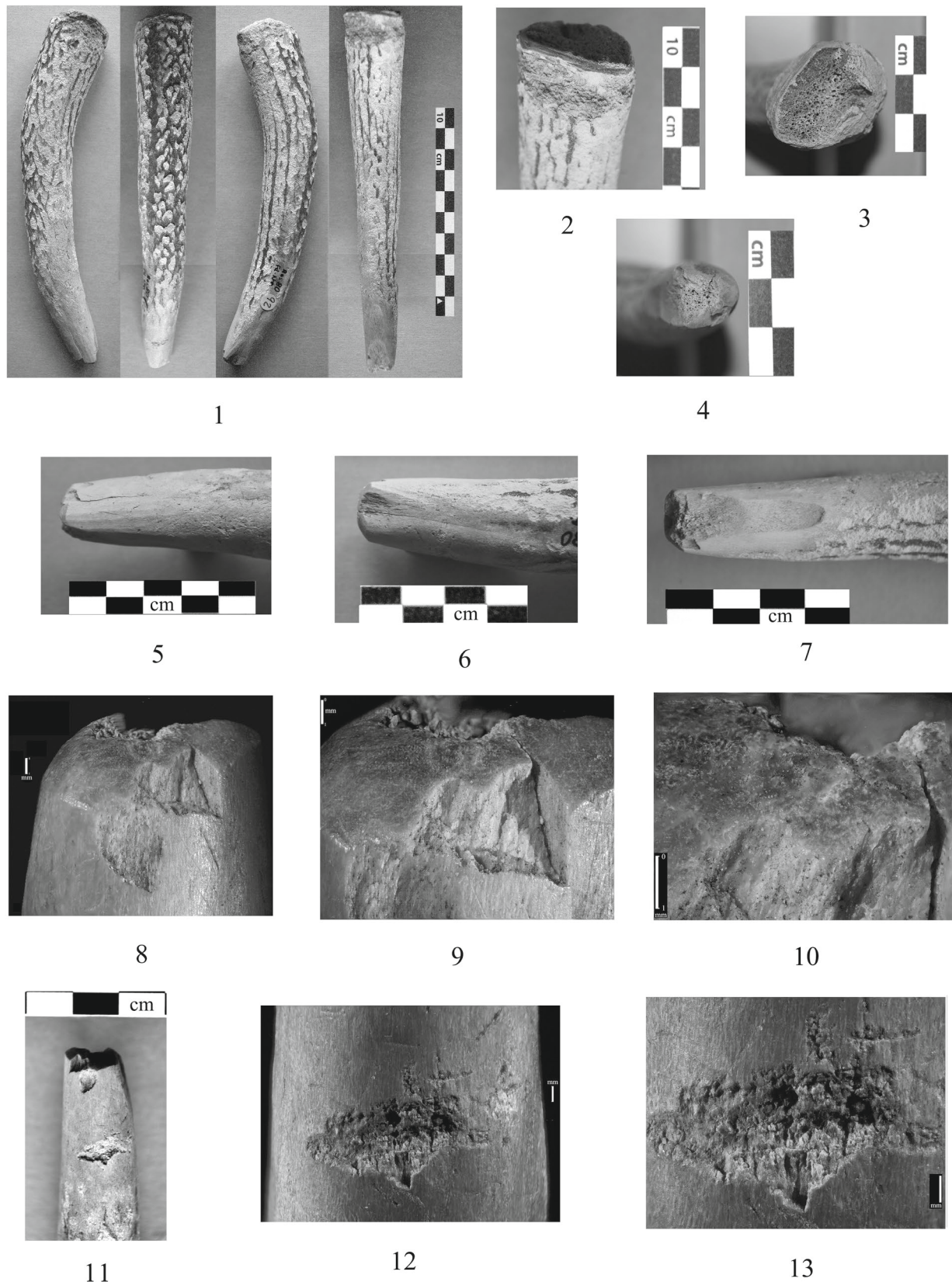
Fig. 10. Punch from Rosenhof (Ros 1980, 92). 1 - general view; 2-3 - butt end; 4 - tip from above; 5-7 - tip from various sides; 8-10 - use-wear traces on the tip in various magnifications; 11-13 - secondary use-wear traces on one side of the working end.
