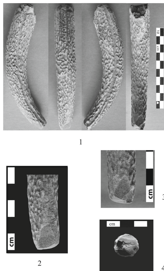
Fig. 7. Punch from Rosenhof (Ros 1970.30, 59). 1 - general view; 2 - tip from convex side; 3 - tip from concave side; 4 - tip from above.
