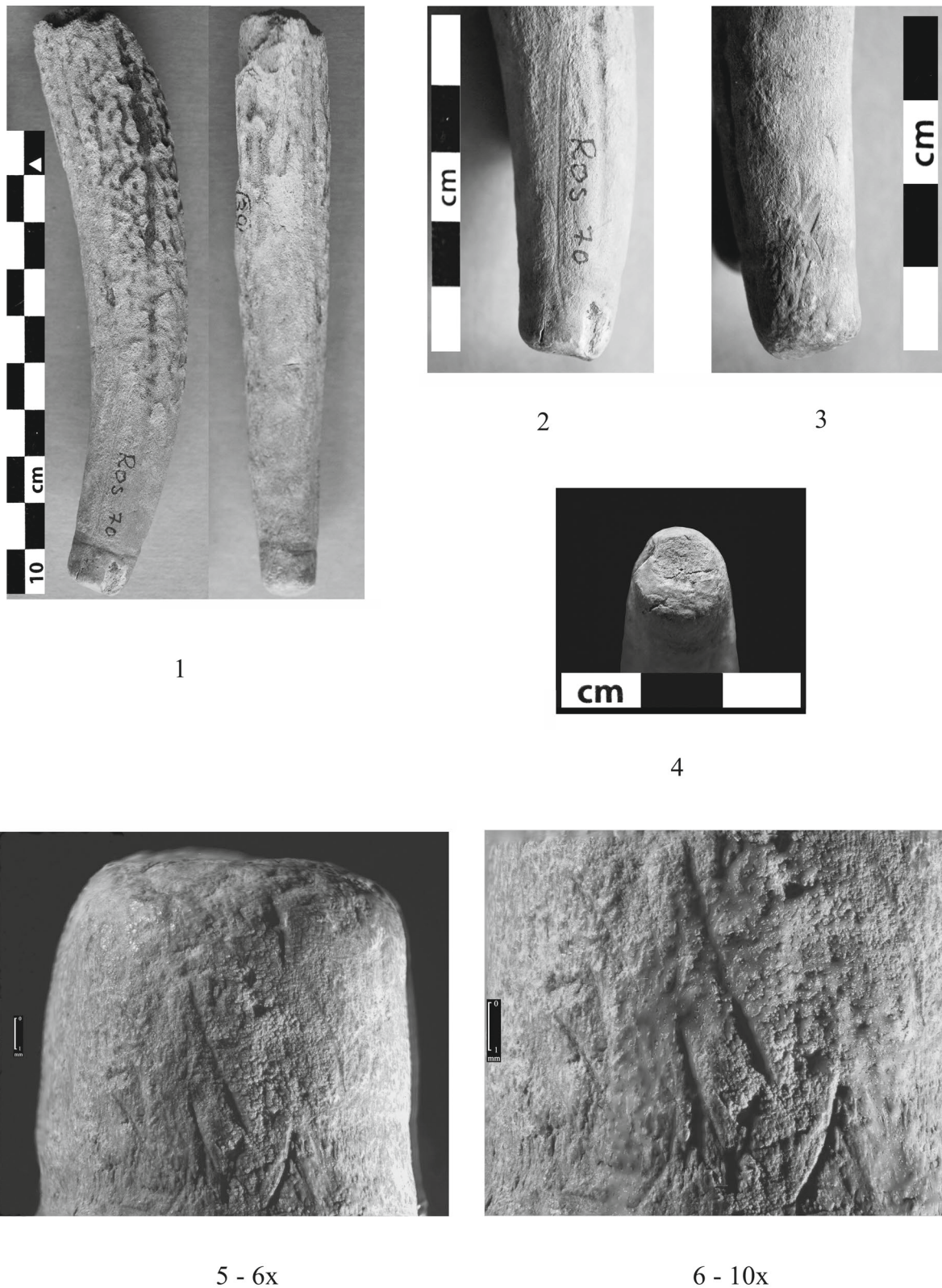
Fig. 8. Punch from Rosenhof (Ros 1970.30). 1 - general view; 2 - tip from convex side; 3 - tip from concave side; 4 - tip from above; 5-6 - use-wear traces on the tip and adjacent areas (5 - 6x, 6 - 10x).
